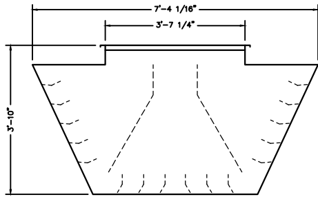
PLAN VIEW
