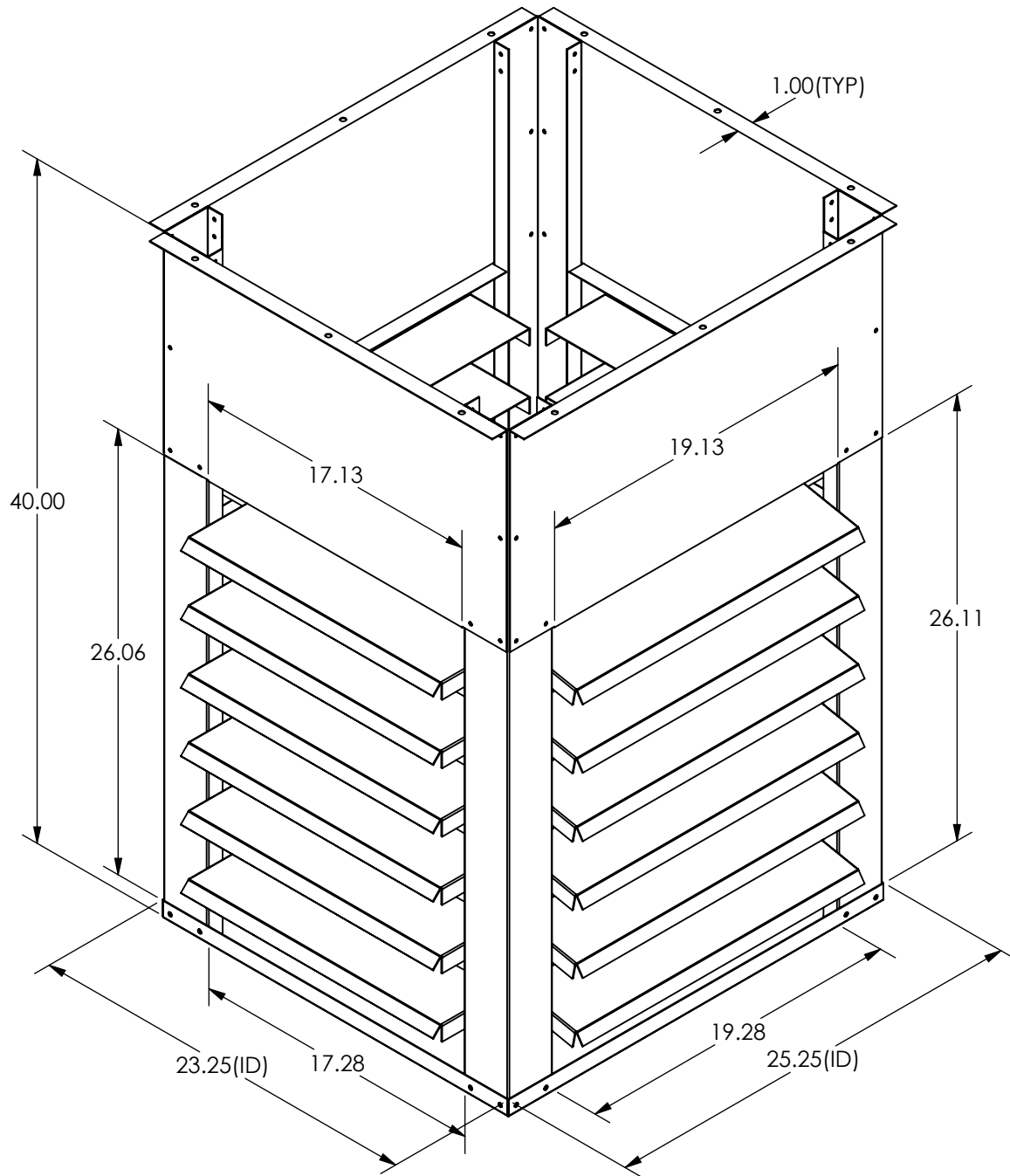
18 and 20 inch blower 3 and 4 way
