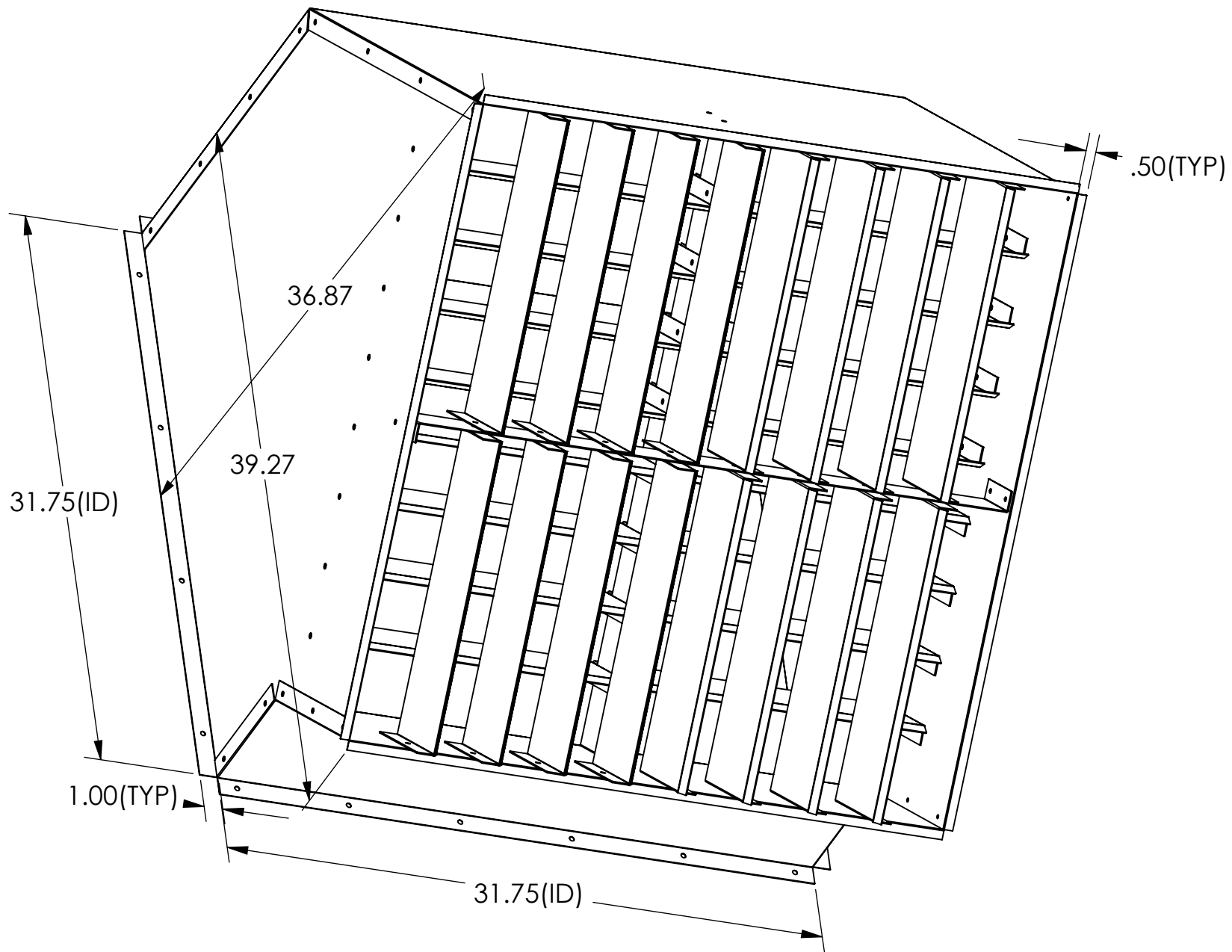
25in Blower 45 Degree
