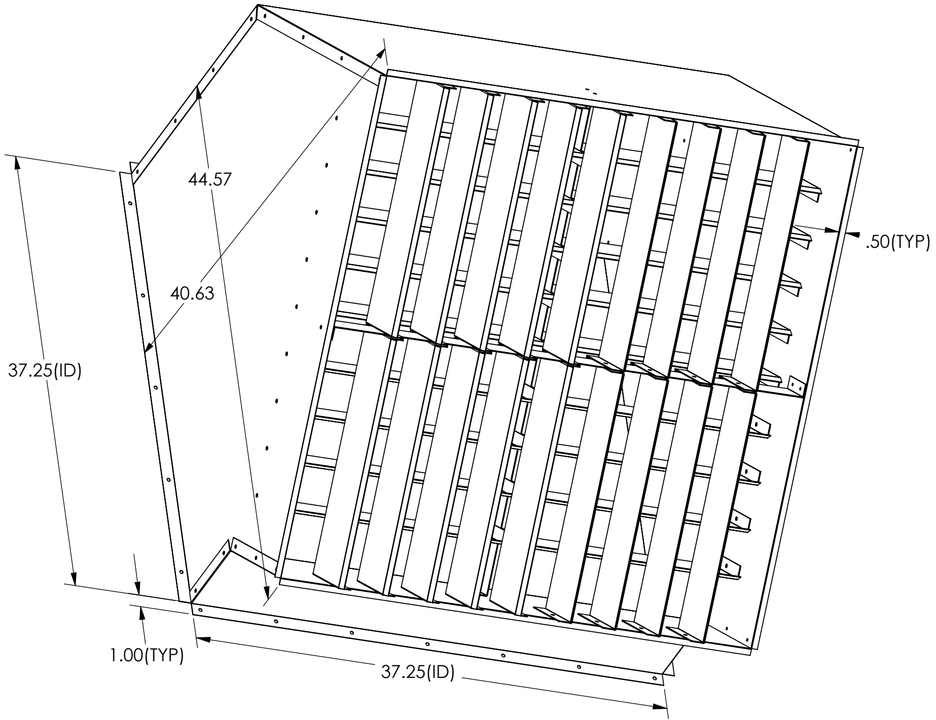
30 inch blower 45 degree
