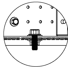
DETAIL B 3/8" HARDWARE DETAILS 16 PLCS SCALE 1 : 4
