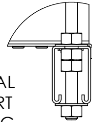
DETAIL A 1/2" ALL THREAD DETAILS 4 PLCS SCALE 1 : 4
