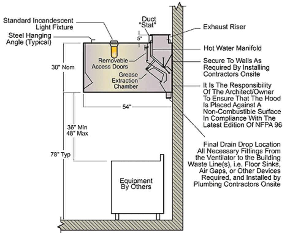
SECTION VIEW MODEL 5430-SCA-N
