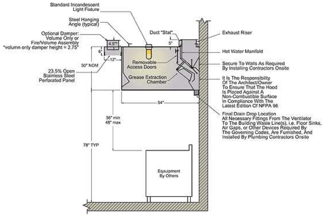
SECTION VIEW MODEL 5430-SCA-N with PSP Accessory
