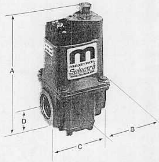
MR410, MR510, MR610
